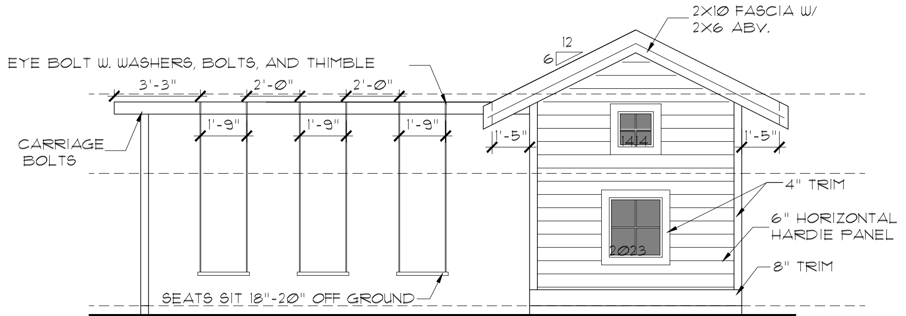
REAR ELEVATION
